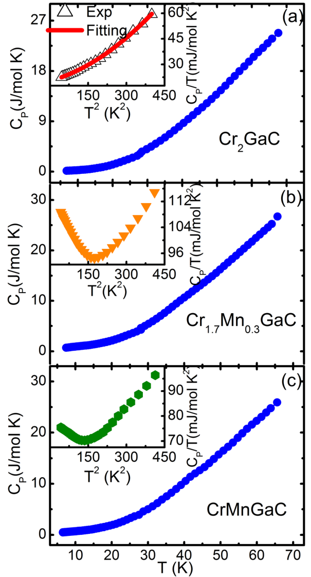
FIG. 7. (a)-(c) Temperature dependent heat capacity C_P(T) at zero field in a temperature of 6.5–65 K for \text{Cr}_{2-x}\text{Mn}_x\text{GaC} ; Inset shows the plot of C_P(T)/T vs. T^2 below 20 K and the solid line represents the fitting results according to Eq. (6).
