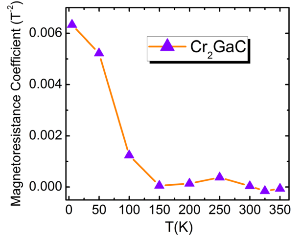
FIG. 6. Temperature dependence of the magnetoresistance coefficient \alpha for \text{Cr}_2\text{GaC} .
