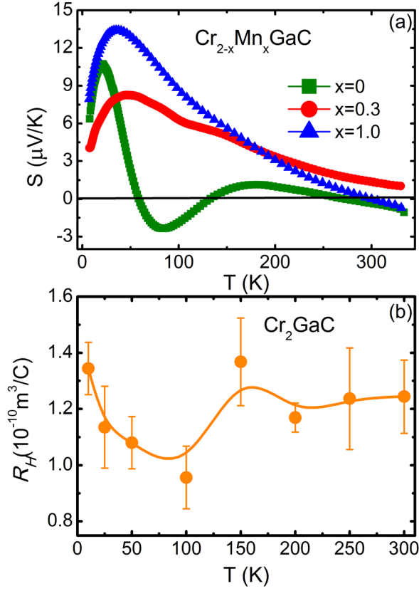
FIG. 5. (a) Temperature dependent Seebeck coefficient at zero magnetic field between 5 and 330 K for \text{Cr}_{2-x}\text{Mn}_x\text{GaC} . (b) Temperature dependent the Hall coefficient for \text{Cr}_2\text{GaC} .
