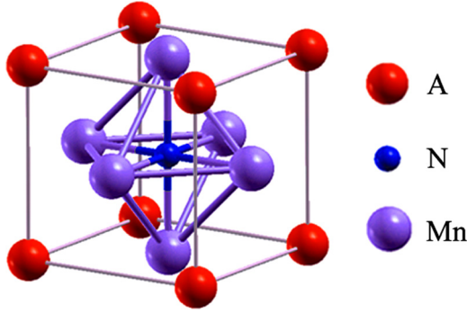
FIG. 1. The schematic structure of manganese nitride antiperovskite \text{AlMn}_3 .
