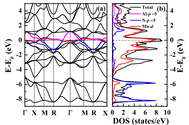
FIG. 3. (a) The band structure of \text{AlMn}_3 with NM state. The colored lines denote the bands cross the Fermi level. (b) The density of states of \text{AlMn}_3 with NM state.
